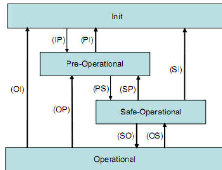
Fig. 5.2- Permitted state transitions of the ESM
